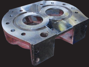
REBUILT MIXER END FRAME WITH NEW CHROME PLATED WEAR PLATES
