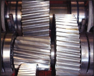
REBUILT GEAR SET FOR AN EXTRUDER APPLICATION
