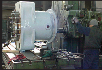
REPAIRS - MACHINING OF HYDRAULIC PRESS CYLINDER
