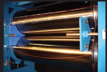
FIELD SERVICE-ROLL GRINDING/ROLL BLOCKING
